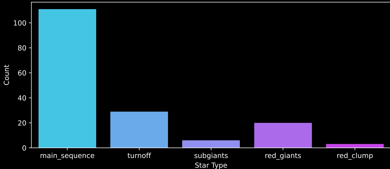
APOGEE DR17 Field: [147+60_MGA] Count plot of Star Type
