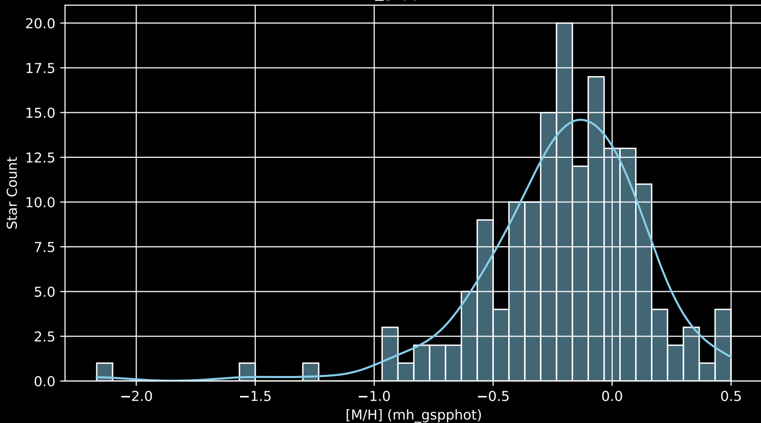
APOGEE DR17 Field: [147+60_MGA [M/H] (mh_gspphot) (n= 166)
