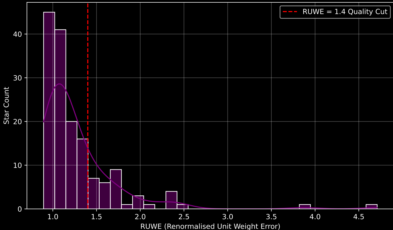
GAPOGEE DR17 Field [147+60_MGA] RUWE Distribution (n= 156)
