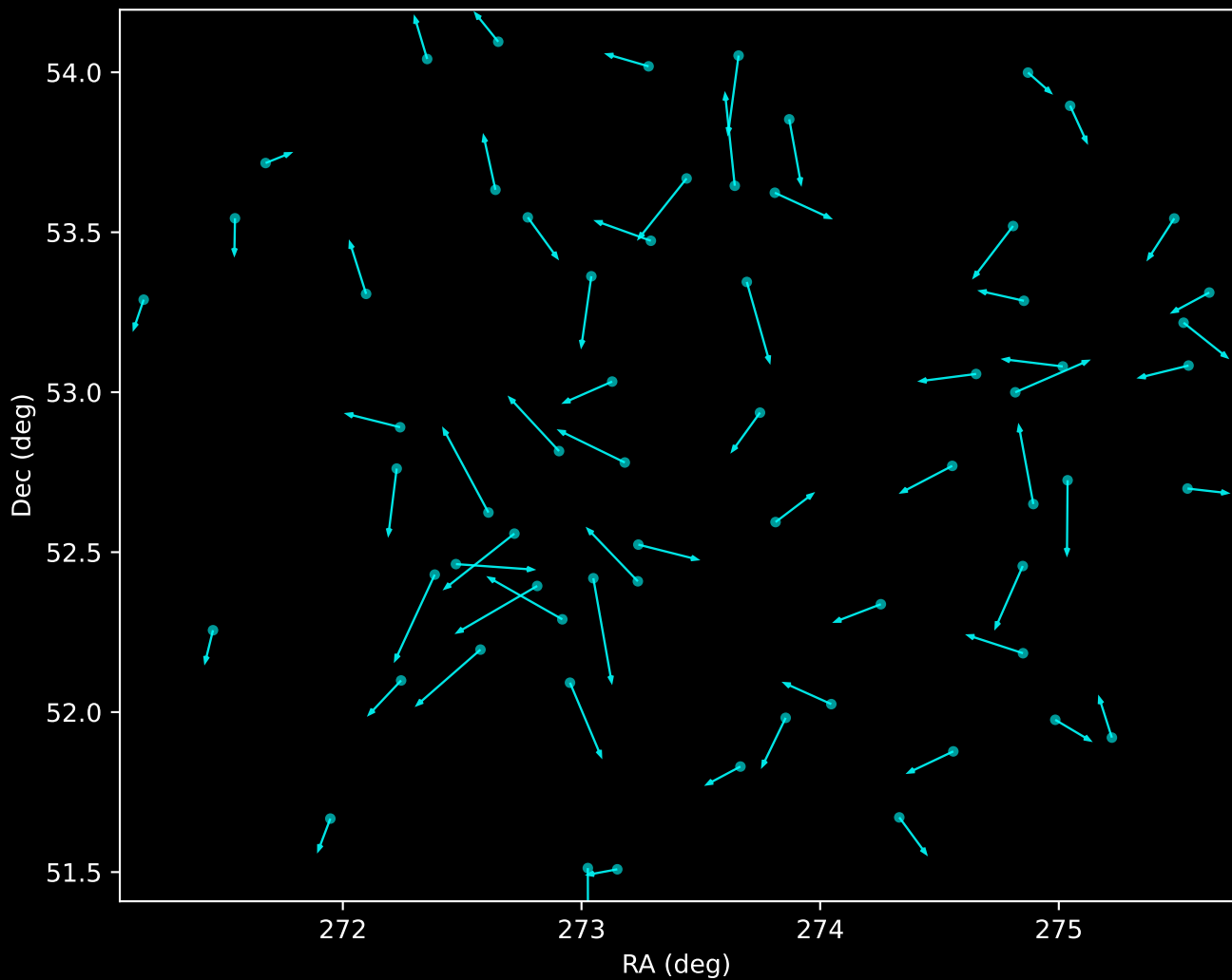
APOGEE DR17 Noise Stream Proper Motion Vectors (n=65)
