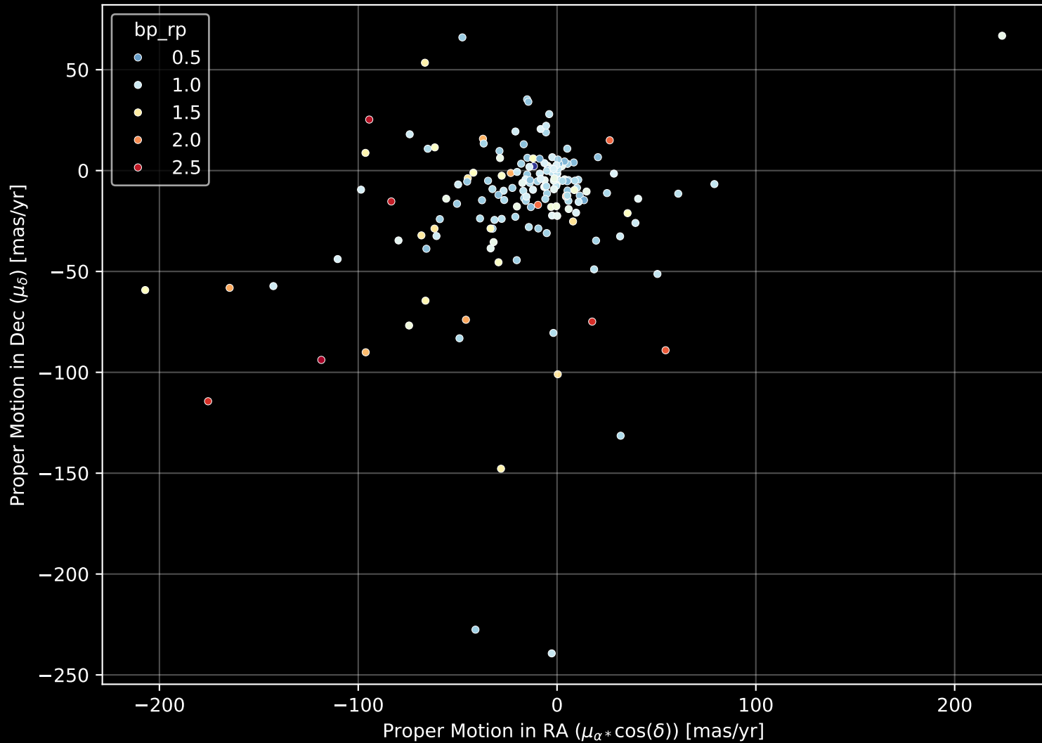
APOGEE DR17 Field: [147+60_MGA] Proper Motion Diagram (n= 169)
