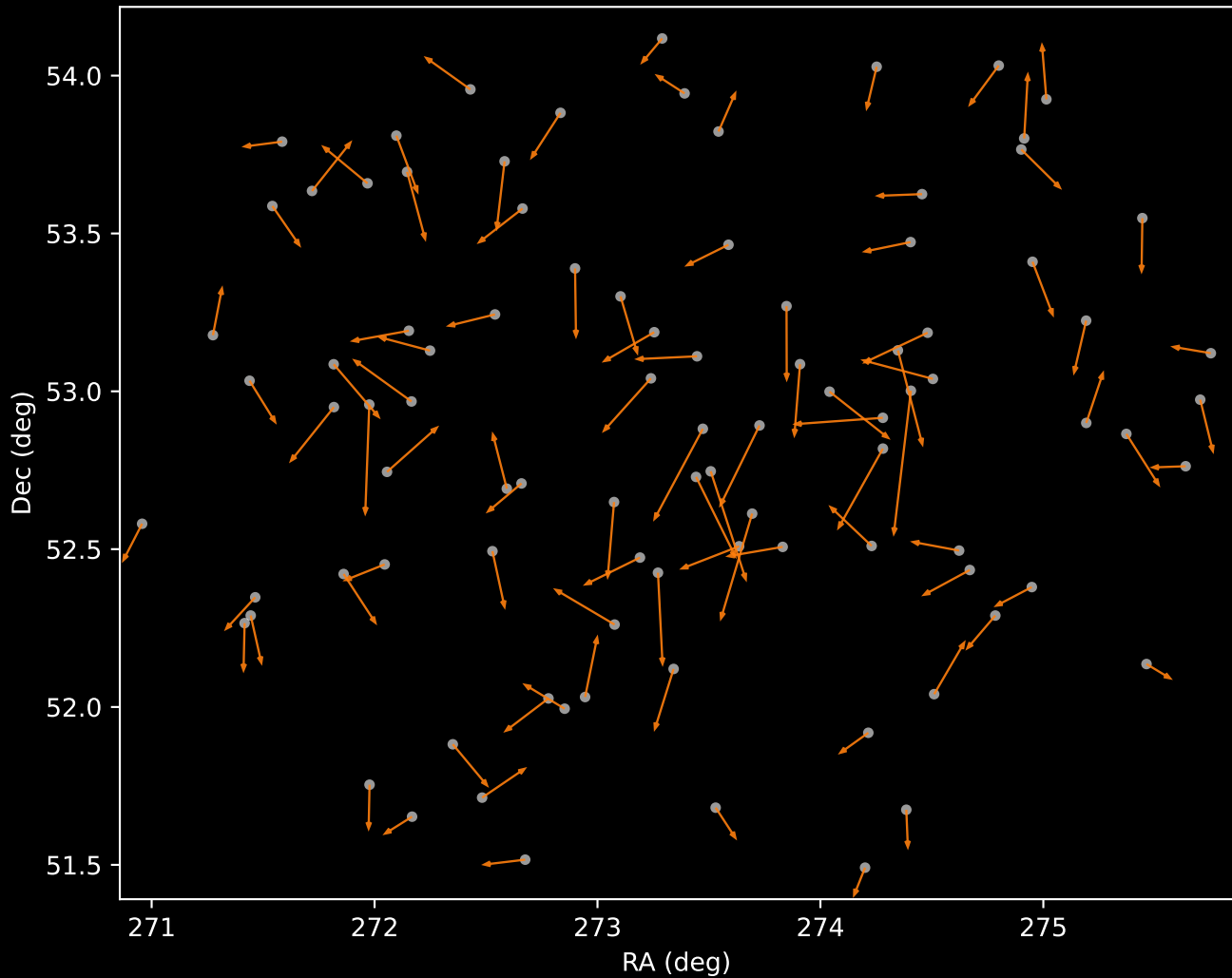
APOGEE DR17 Cluster 2 Proper Motion Vectors (n=93)
