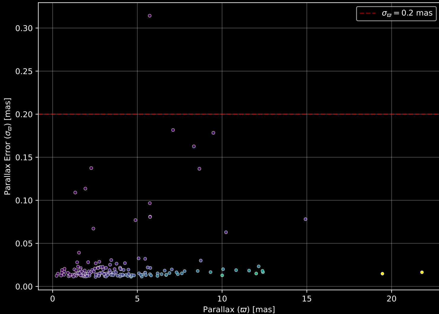
APOGEE DR17 Field: [147+60_MGA] Parallax Quality (n= 169)
