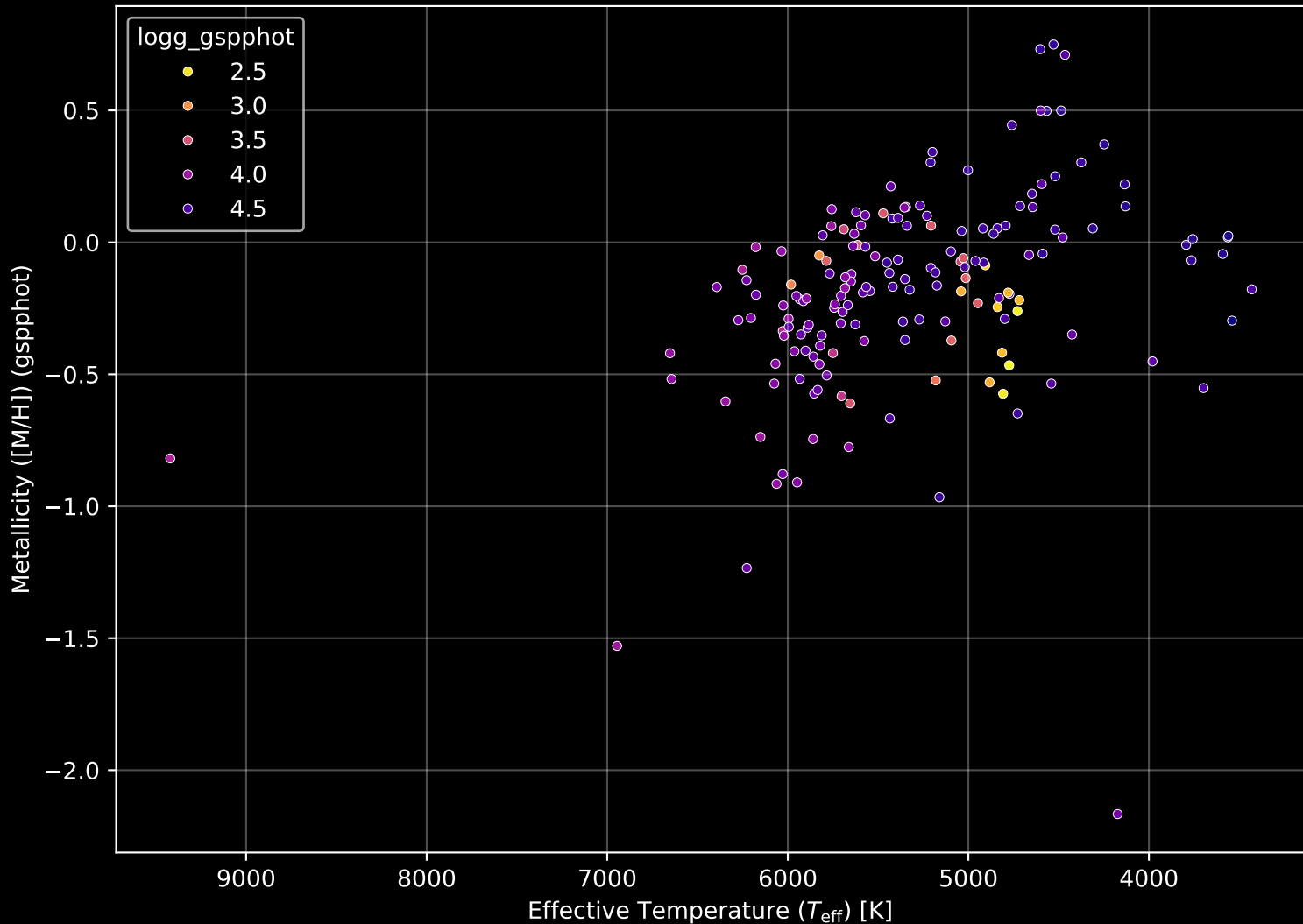
APOGEE DR17 Field: [147+60_MGA] Stellar Population Parameters (n= 169)
